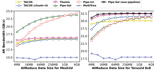
Fig. 9. AllReduce bandwidth comparison against MultiTree on 8x8 2D Mesh and 8x8 2D Torus topologies. The black curve represents Pipe-Sol with the pipeline constraints relaxed (i.e., equivalent to a non-pipelined shortest-path strategy).
