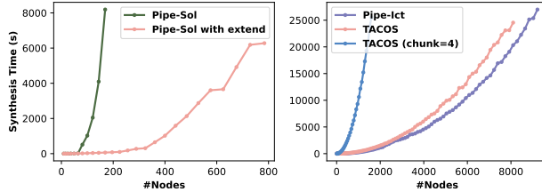
Fig. 12. Synthesis time of different approaches for various-sized homogeneous 2D Meshes. Pipe-Ict exhibits \Theta(n^2) synthesis time complexity, where n is the number of nodes.
